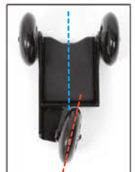
Stand roller tire has a camber angle for easy to move the bike.
